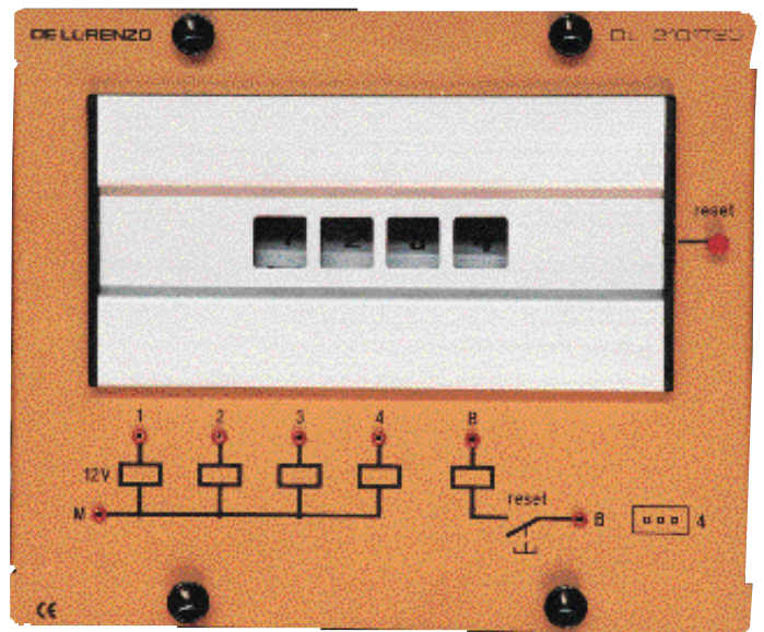
DL 2101T23 TAG SIGNALLING Board with four tags; supplied with reset button. Operating voltage: 12 Vac.
