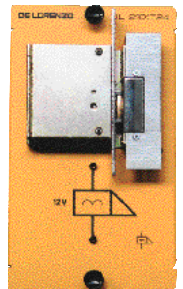
DL 2101T24 DOOR OPENER Lock with electromagnetic control. Operating voltage: 12 Vac, 18 VA.
