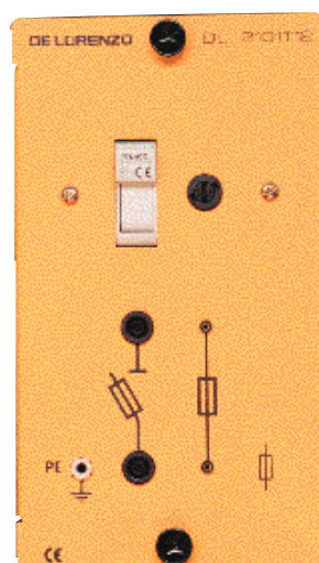
DL 2101T12 FUSES HOLDER Isolator with cartridge fuse 2 A, 500 V. Holder with miniature fuse 2 A, 250 V.
