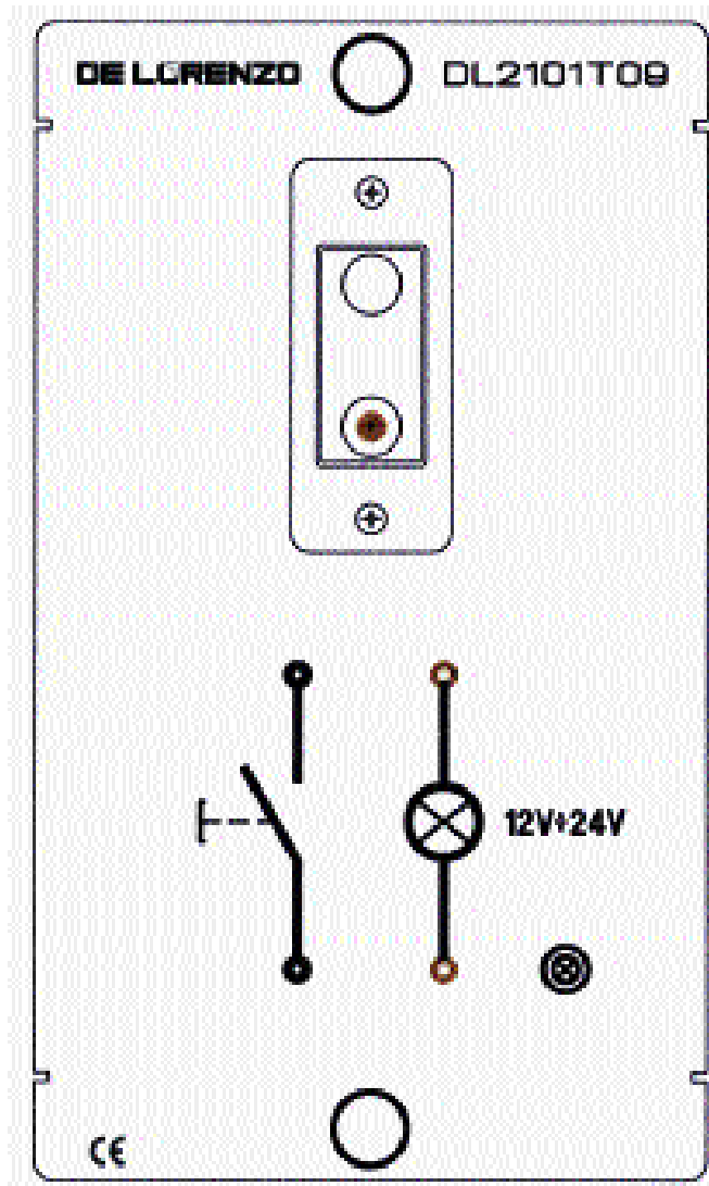
DL 2101T09 ILLUMINATED PUSHBUTTON Single pole switch 250Vac, 10A. Supplied with 24 Vac pilot lamp.
